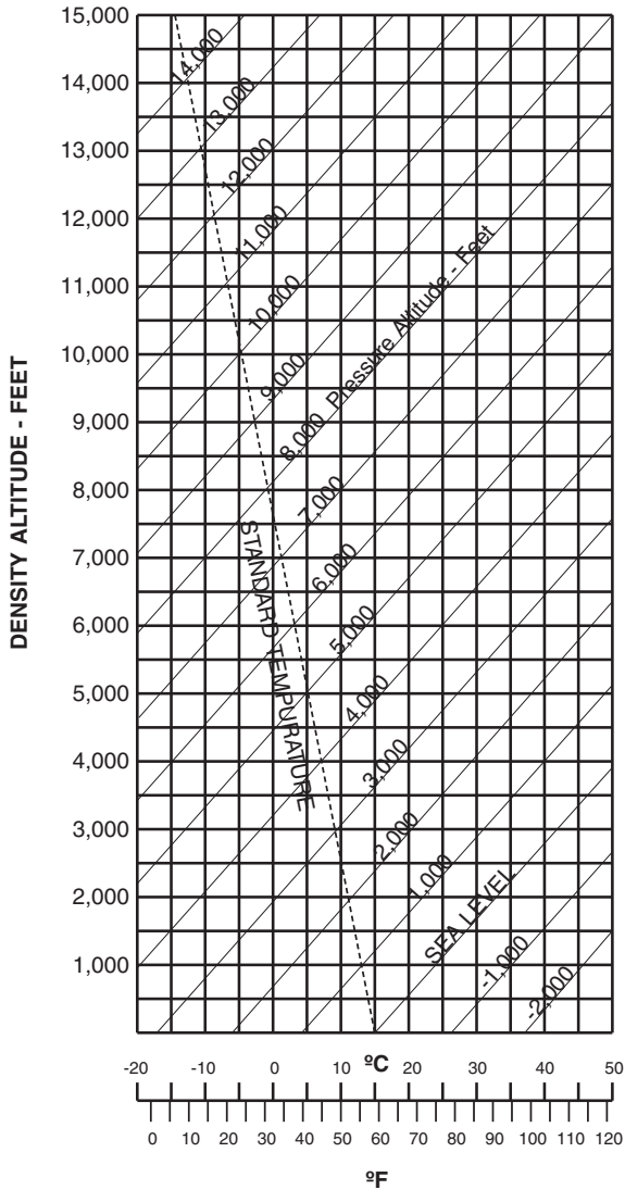
Figure 5-1 Density Altitude Chart
