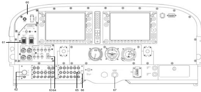
Figure 7-2 Example of Instrument Panel (G1000 with Engine Indication System)
